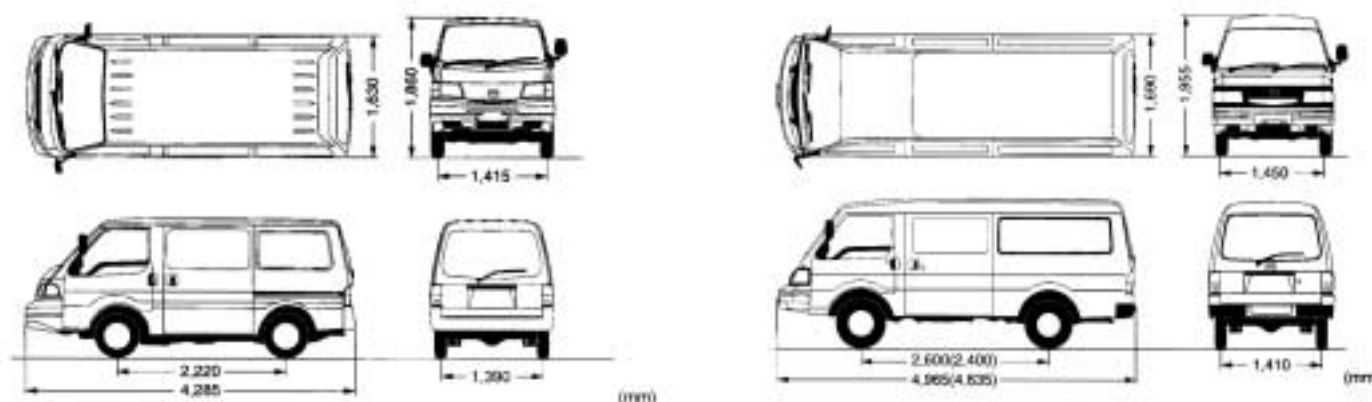
1.8 Short wheel-base
